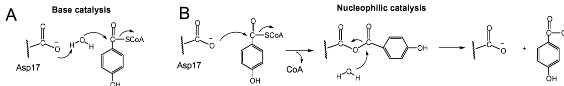
FIGURE 7: Mechanisms for thioesterase catalysis with Asp17 serving in the role of (A) general base or (B) nucleophile.
