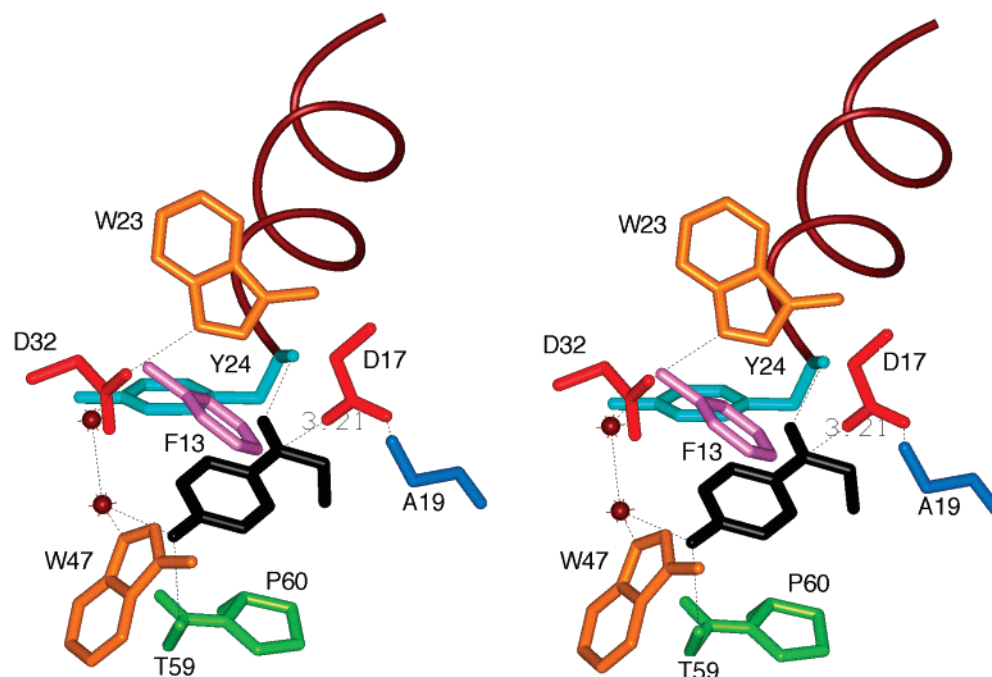
FIGURE 6: Stereodiametric of the catalytic site of the wild-type 4-HBA-CoA thioesterase with 4-hydroxyphenacyl-CoA truncate bound (black) generated using Insight II and the coordinates reported in ref 13.
